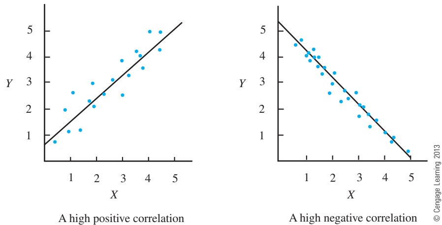
FIG-1-3 Graphs of high positive and high negative correlations
